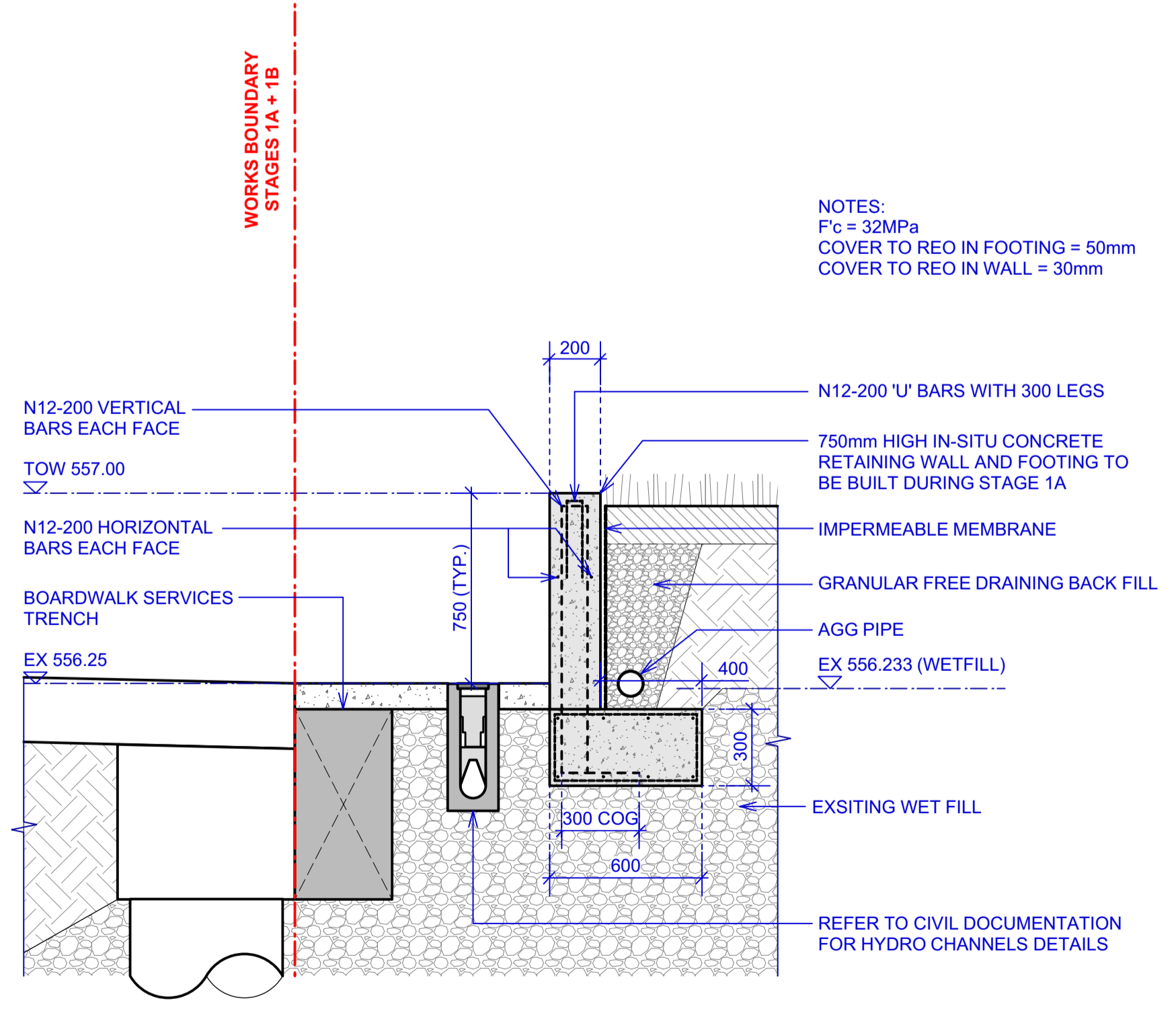
2 DETAIL SECTION - WA02 RETAINING WALL ALONG BOARDWALK (STAGE 1A) Scale: 1:20
