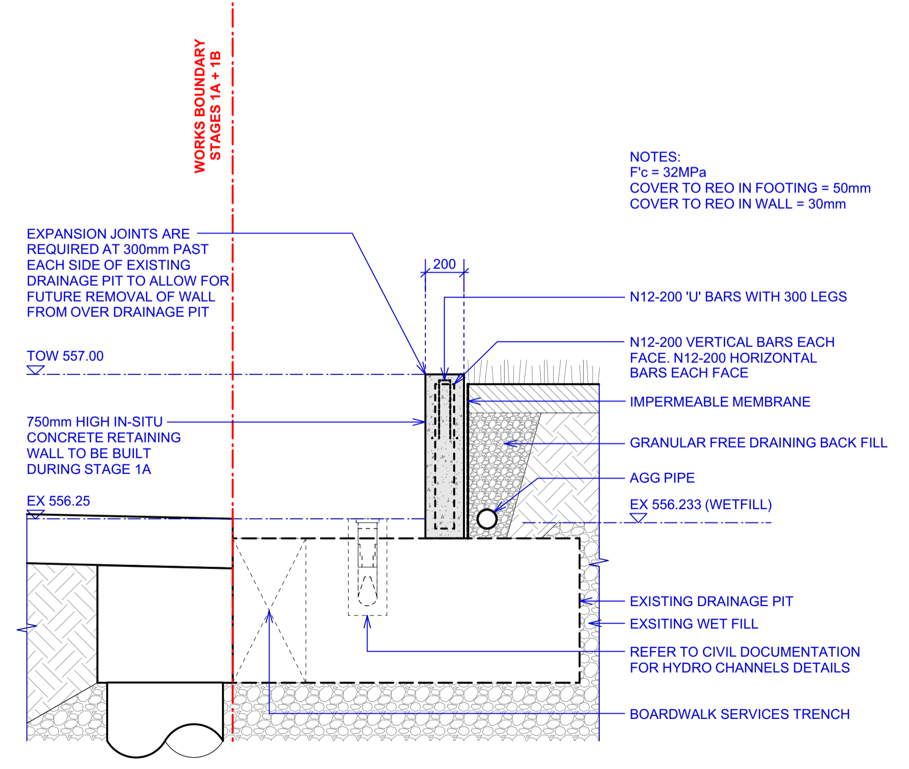
3 DETAIL SECTION - WA02 CROSS EXISTING DRAINAGE PIT (STAGE 1A) Scale: 1:20
