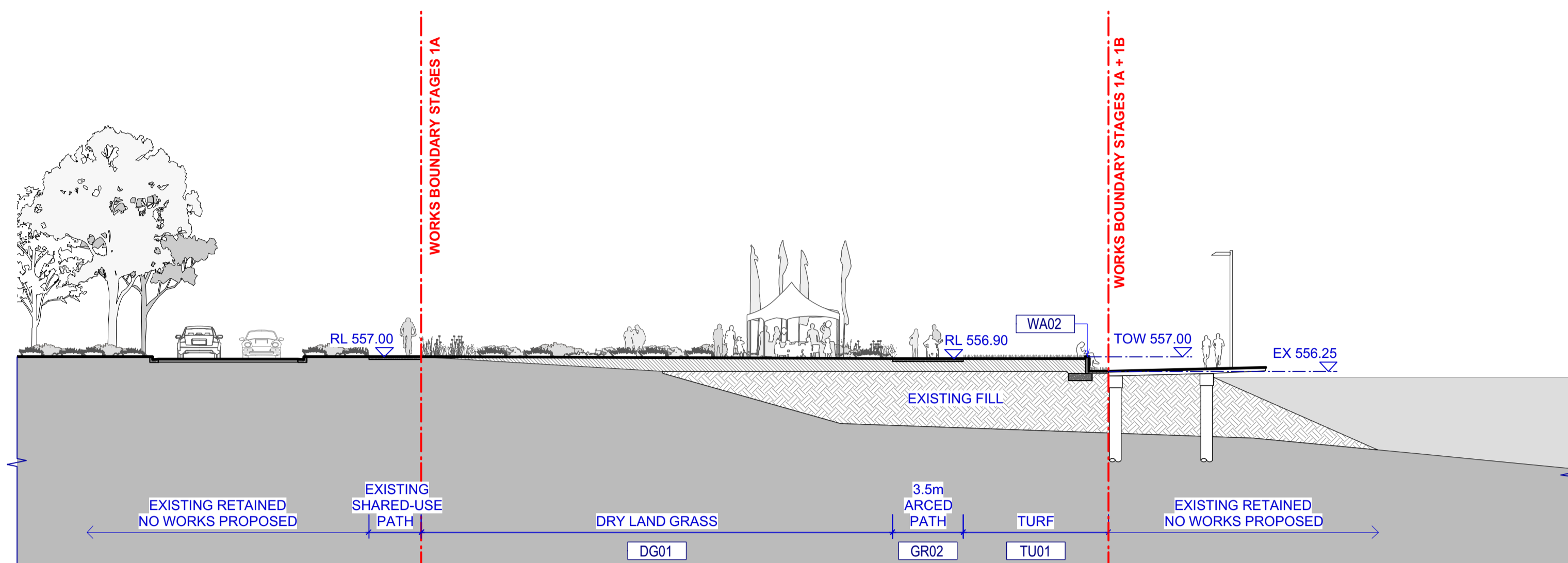
1 SITE SECTION - ARRIVAL PLAZA (STAGE 1A) Scale: 1:200
