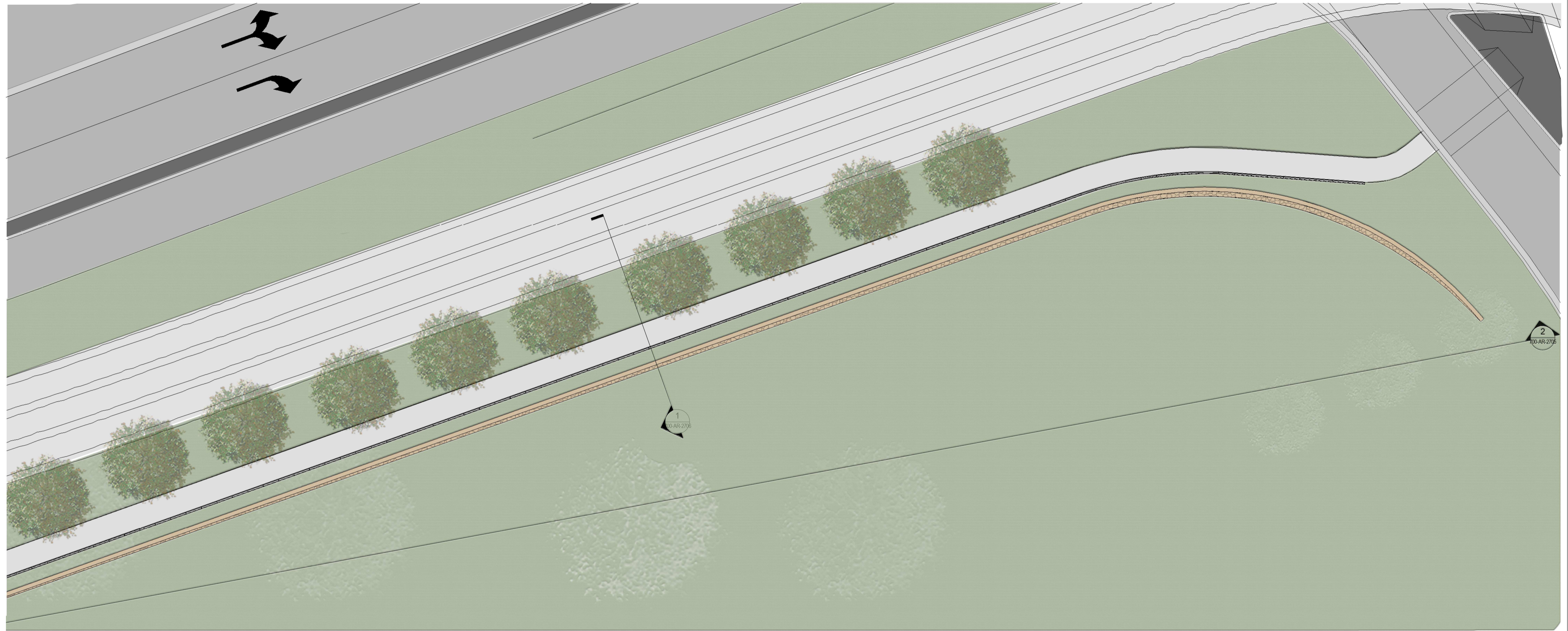
1 RETAINING WALL PLAN B - CNR FEDERAL HIGHWAY & FLEMINGTON ROAD Scale: 1 : 125
