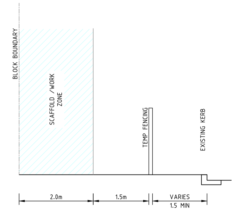
TYPICAL VERGE SECTION
